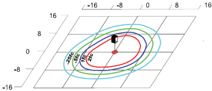
BSL-Q-F-R3-15L-QT-50K Mounting Height = 3.5ft
