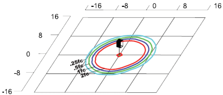
BSL-Q-F-AR-15L-QT-50K Mounting Height = 3.5ft
