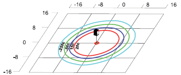
BSL-Q-F-R5-15L-QT-50K Mounting Height = 3.5ft
