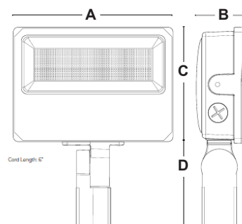
Slip Fitter Mount
