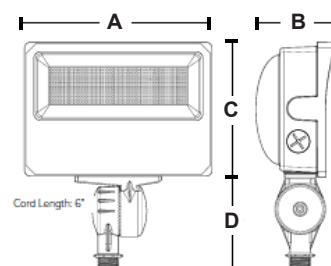
Knuckle Mount
