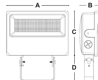
Yoke Mount
