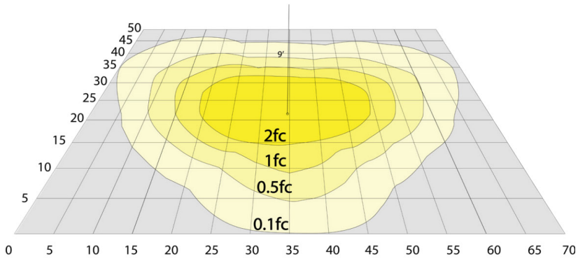
70W, 5000K Area 50'x 70' Mounting Height: 9'
