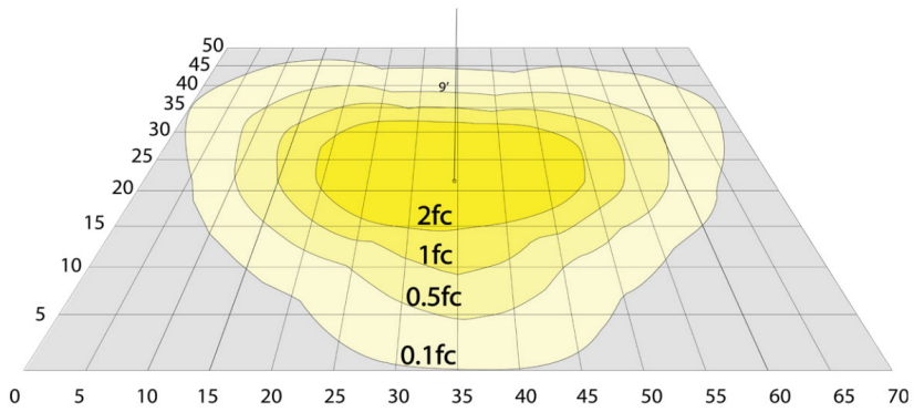
50W, 5000K Area 50'x 70' Mounting Height: 9'
