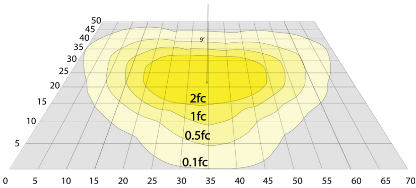
60W, 5000K Area 50'x 70' Mounting Height: 9'
