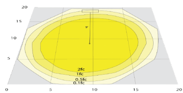
OC8-R2-DL (5000K, 20' x 20', Mounting Height: 9')
