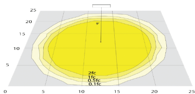
OC8-R2-UD (5000K, 25' x 25', Mounting Height: 9')
