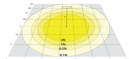
OC8-R4-UD (5000K, 35' x 35', Mounting Height: 9')
