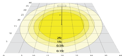
OC8-R3-DL (5000K, 40' x 40', Mounting Height: 9')
