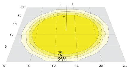
OC8-R3-UD (5000K, 25' x 25', Mounting Height: 9')
