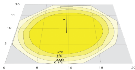
OC8-S3-DL (5000K, 20' x 20', Mounting Height: 9')
