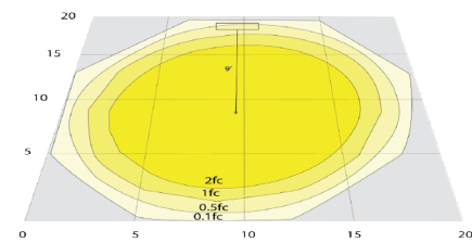
OC8-R5-UD (5000K, 20' x 20', Mounting Height: 9')
