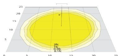
OC8-R1-UD (5000K, 25' x 25', Mounting Height: 9')
