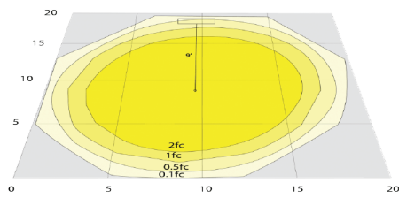
OC8-R3-DL (5000K, 20' x 20', Mounting Height: 9')
