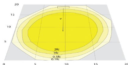
OC8-S1-DL (5000K, 20' x 20', Mounting Height: 9')
