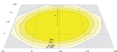
OC8-R1-DL (5000K, 20' x 20', Mounting Height: 9')
