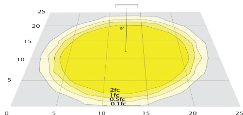
OC8-S1-DL (5000K, 25' x 25', Mounting Height: 9')
