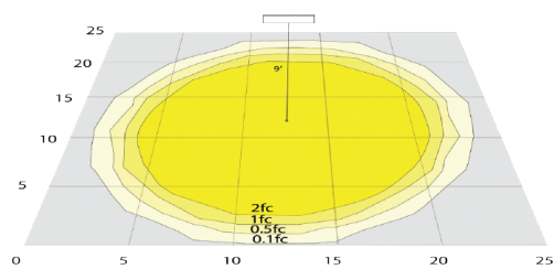
OC8-S3-UD (5000K, 25' x 25', Mounting Height: 9')
