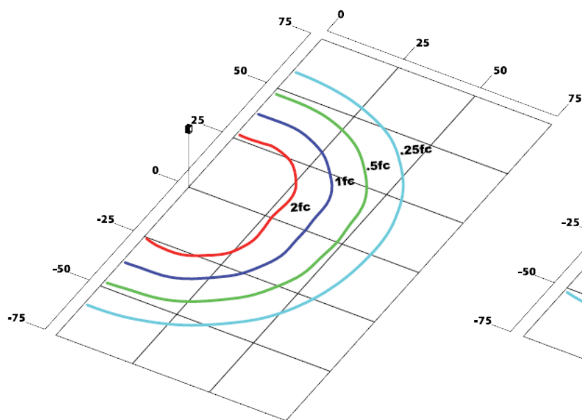
PT5-Q-176L-QT-50K-T5-CL Mounting Height = 25ft
