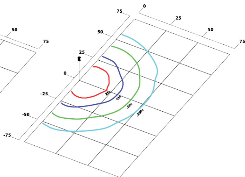
PT5-Q-100L-QT-50K-T3-CL Mounting Height = 25ft
