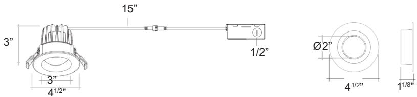
RDL4-EN (18W)
