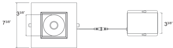
RDL6-EN (Square)
