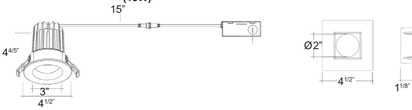
RDL6-EN (Square)
