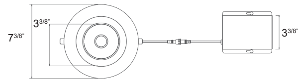
RDL6-EN (Round)
