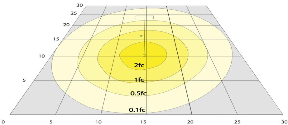
9W 5000K, Area 30'x30' Mounting Height 9'
