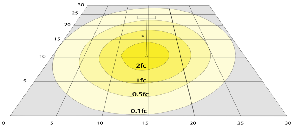
9W 5000K, Area 30'x30' Mounting Height 9'
