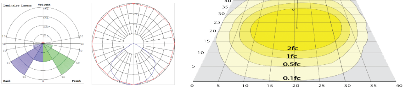
SST1-W-6X1L-QT-MCT 30W, 4000K, 50'X40' Area, 9' Mounting Height BUD Rating: B1-U2-G1
