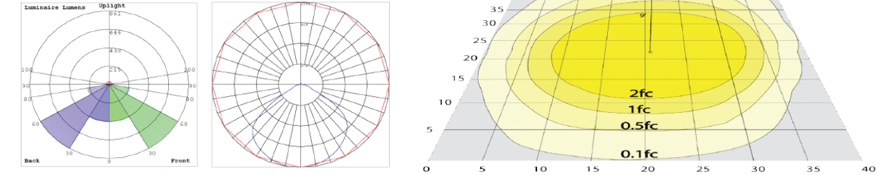
SST1-W-4X1L-QT-MCT 30W, 4000K, 50'X40' Area, 9' Mounting Height BUD Rating: B1-U2-G1
