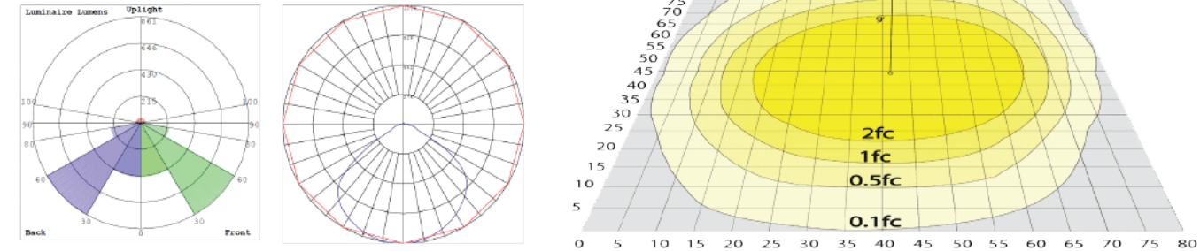
SST1-W-8X1L-QT-MCT 60W, 4000K, 100'X80' Area, 9' Mounting Height BUD Rating: B1-U2-G1
