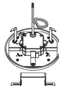
Snap-in Mounting Bracket Over a Plastic or Metal 4/O J-Box
