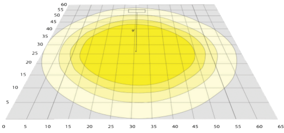
WP53.5-W-2L Area 60' x 65' Mounting Ht: 9'
