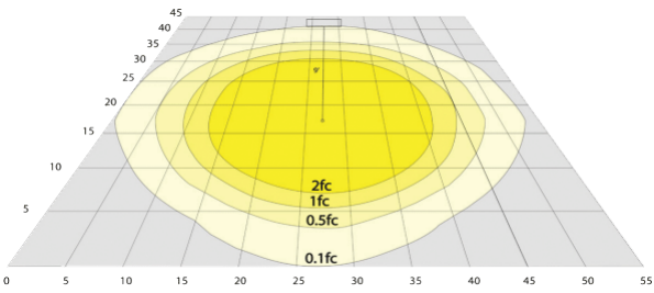
WP53.5-W-1L Area 45' x 55' Mounting Ht: 9'
