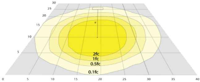
WP53.5-W-12L Area 30' x 40' Mounting Ht: 9'
